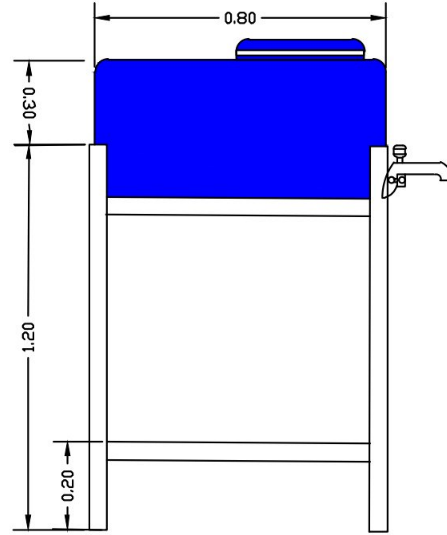
Side view
